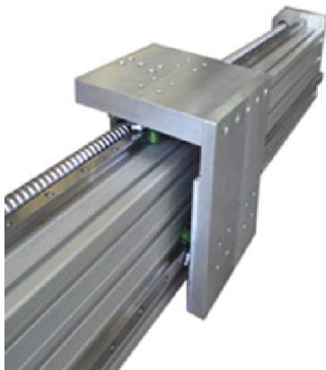
Screw Shaft and Applications Studs
