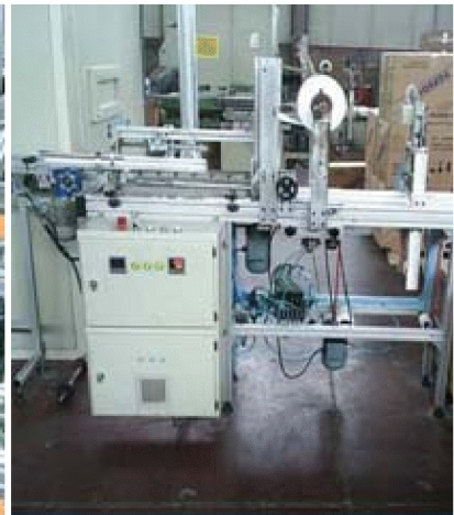
Pet Cup Machine Views 3
