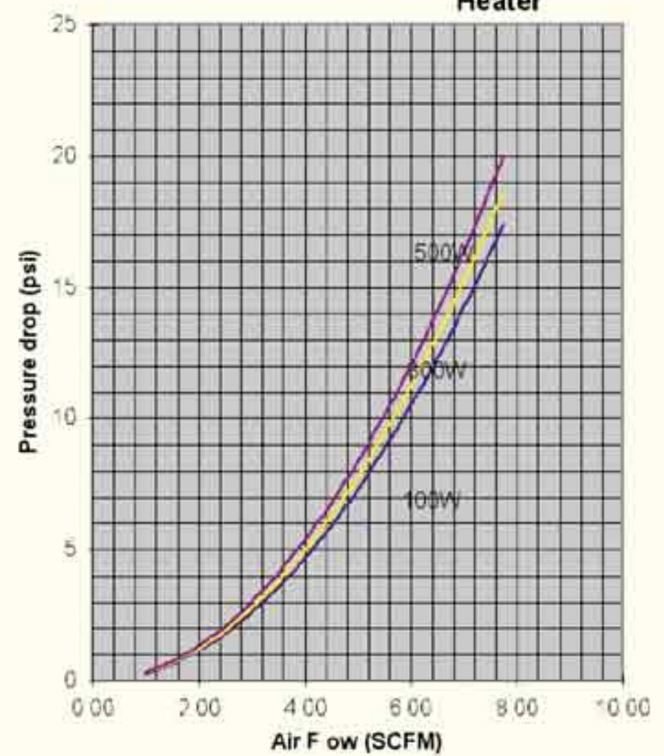
Triple Pass Heater
