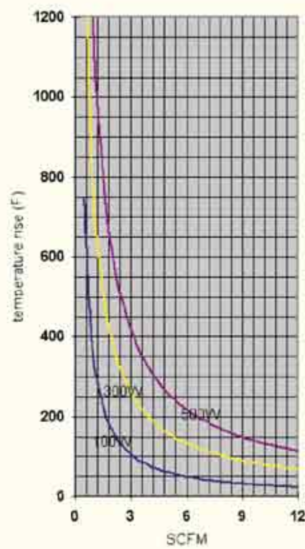
Triple Pass Heater
