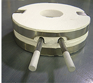
High Temperature Sleeve Heater Part # SLH1.5
