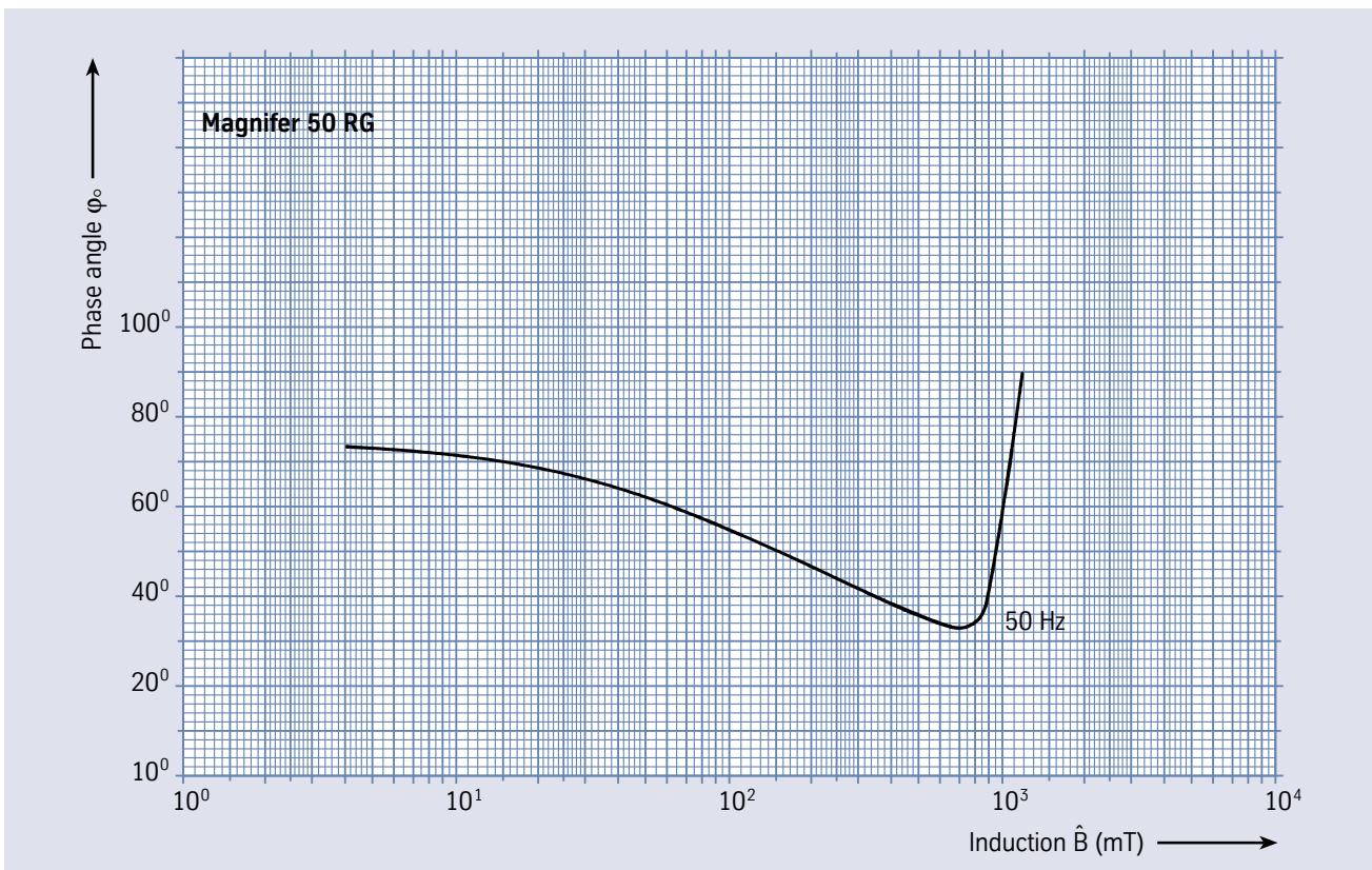
Fig. 5 – Phase angle \phi_0 of Magnifer 50 RG, measured using toroidal tape-wound cores of 0.2 mm strip thickness.
