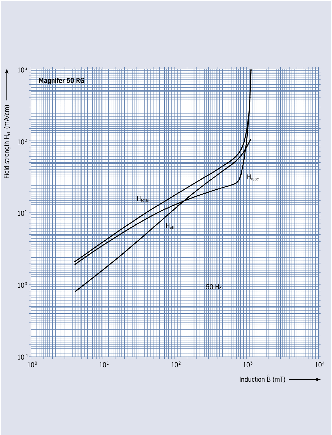
Fig. 6 – Components of the magnetization curve of Magnifer 50 RG, measured using toroidal tape-wound cores of 0.2 mm strip thickness.
