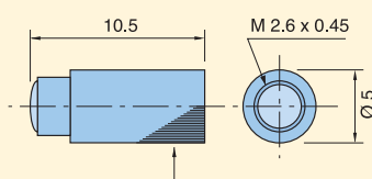
LENTE MOD. AT-4101/ACF000006 LENS VIEWER AT-4101
