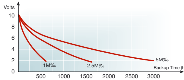
Figure 36. 1.0F-LV Series
