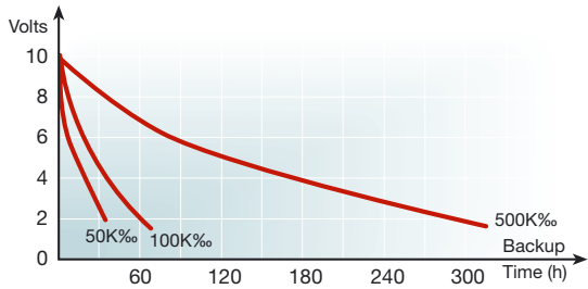
Figure 35. 1.0F-LV Series
