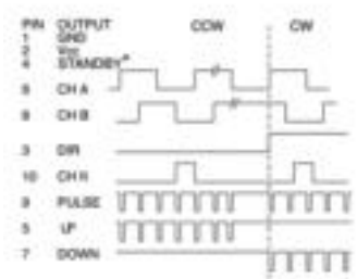
* For operation, connect STANDBY (4) to Vcc (2)
