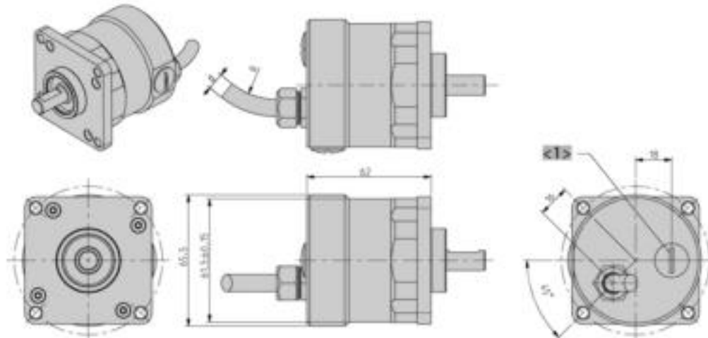
AC 61 Connection cable "A" Interface: BiSS, SSI, ST-/ MT-Parallel, SSI-P
